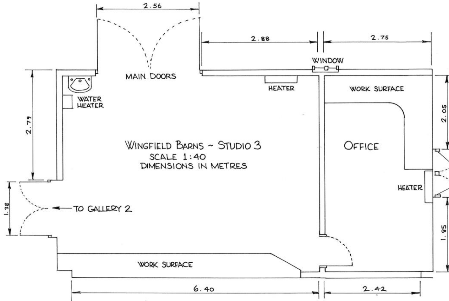
DRAWING X501 - FLOORPLAN (NO CHANGES PROPOSED)
